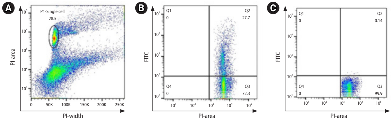
Supplementary Figure 1. (A) Non-clumped cells are gated. (B) Cells containing fragmented DNA were measured from the single cells by propidium iodide (PI)-area positive and fluorescein (FITC) positive (Q2). (C) Negative control without adding terminal deoxynucleotidyl transferase enzyme.
